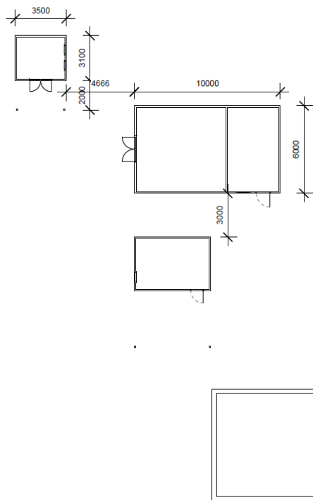
Figur 2. Plantegning.
